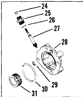
PARKING BRAKE WITH SPEED GEAR
