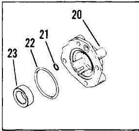
PARKING BRAKE LESS SPEED GEAR
